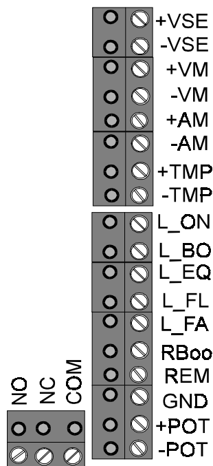
Illustration 8. Location of the external connections.
