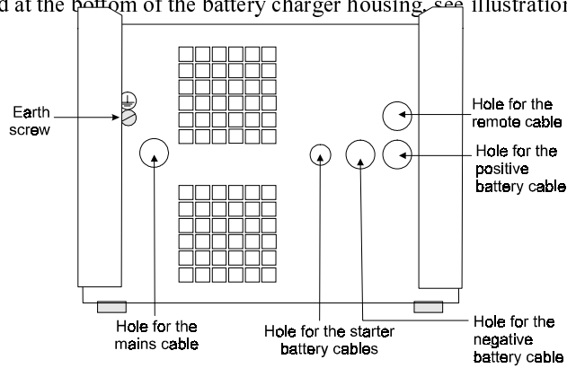
Illustration 2, Location of the charger connection holes
